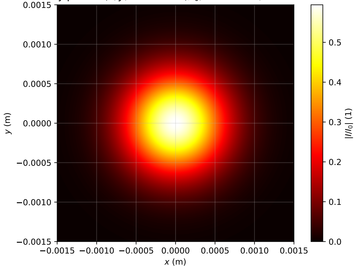
Intensity profile I(x, y, z = 1.990\text{m})/I_0 , \text{Pin}=0.2\text{Pcr} , artificial time
